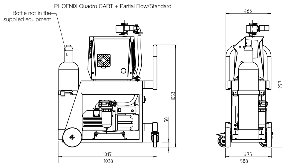
Dimensional drawing PHOENIX 4 Cart with standard castors (Dimensions in mm)
