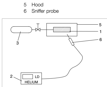
Integral method (search gas accumulation) Search gas overpressure in the test object
