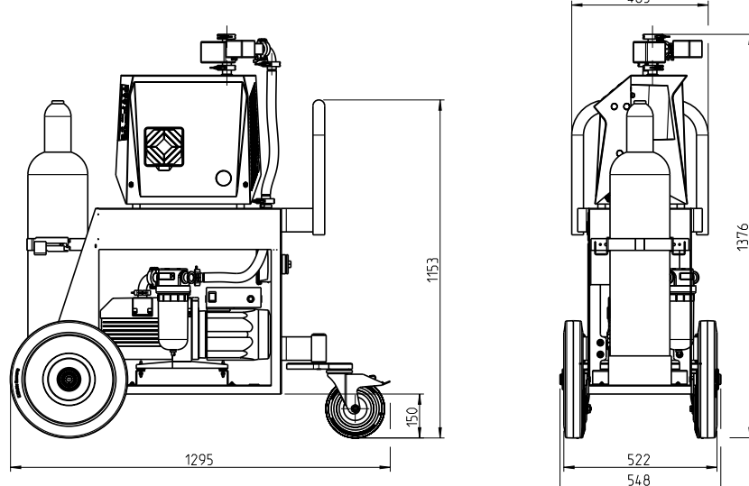
PHOENIX Quadro CART + Partial Flow/Off-Road
